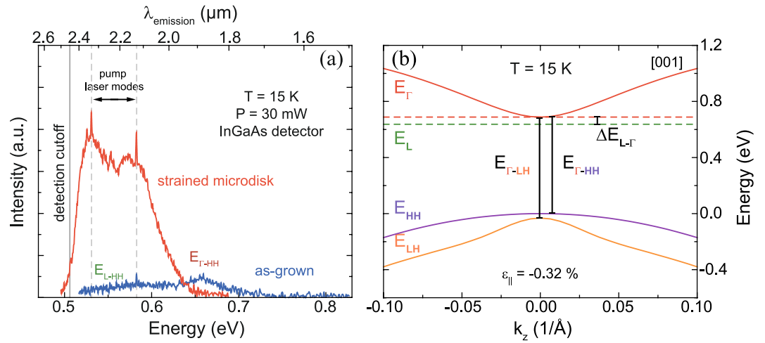
Figure 2. (a) PL spectra of the as-grown \text{Ge}_{0.937}\text{Sn}_{0.063} layer (blue) and a strained 6\mu\text{m} diameter microdisk (red). The sharp peaks indicated by black arrows stem from the pump laser beam. (b) Band dispersion of the as-grown alloy in the [001] direction at 15 K. The lowest band edge of the indirect L-valley is indicated by dashed green lines.
