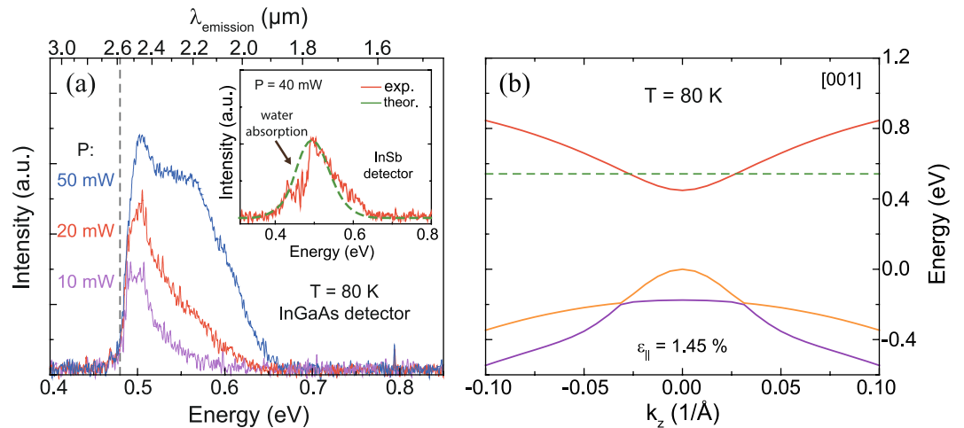
Figure 3. (a) PL spectra of the 6\mu\text{m} diameter disk measured under different excitation power. The inset shows the measurement at 40 mW performed with an LN 2 cooled InSb detector. (b) Band dispersion of the micro disk under 1.45% tensile strain at 80 K.
